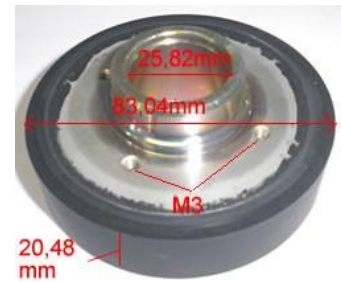
BLACK ROLLER TO PRESS THE PICK NISSAN LW/TSU
