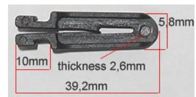
HOOK REGGIL.NISSAN/TSUD. 39,2X10X5,8X2,6 DH-S0300-0
