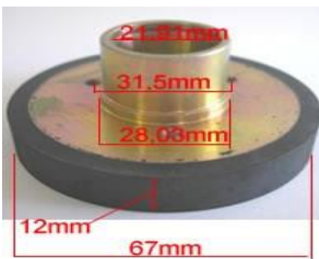
ROLLER FOR FEEDER TSUD.ZW/NISSAN LW/TOYOTA
