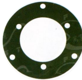
SPRING BUSHING Φ95XΦ165X1.2
